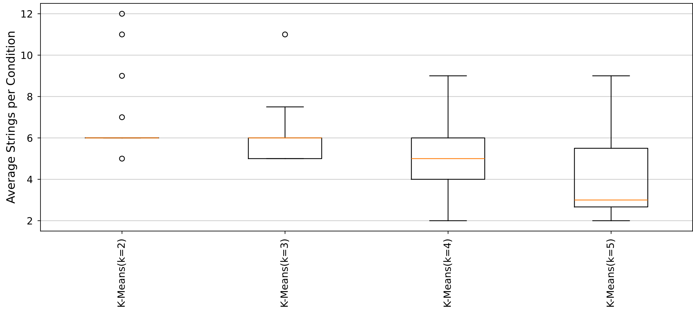
YARA Rules Average Strings per Condition Distribution (Cluster41_Size5 dataset)
